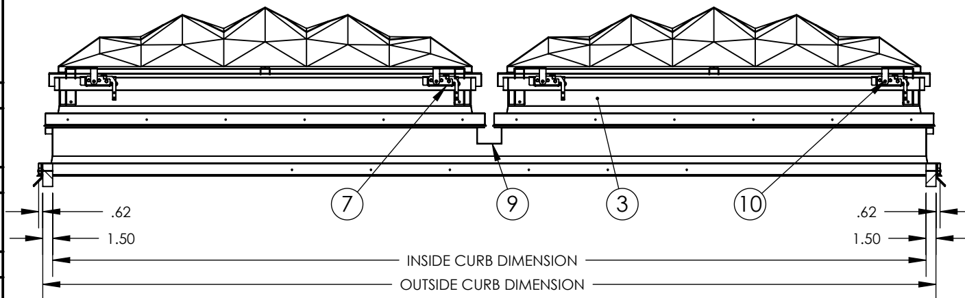
SECTION VIEW SCALE 1 : 20
