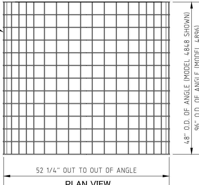
PLAN VIEW SCALE: 3/4" = 1'-0"
