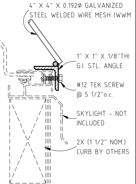
SECTION "A-A" HALF SCALE
