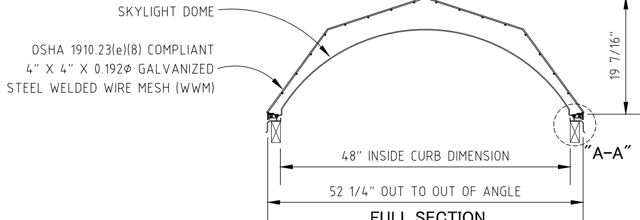
FULL SECTION SCALE: 3/4" = 1'-0"
